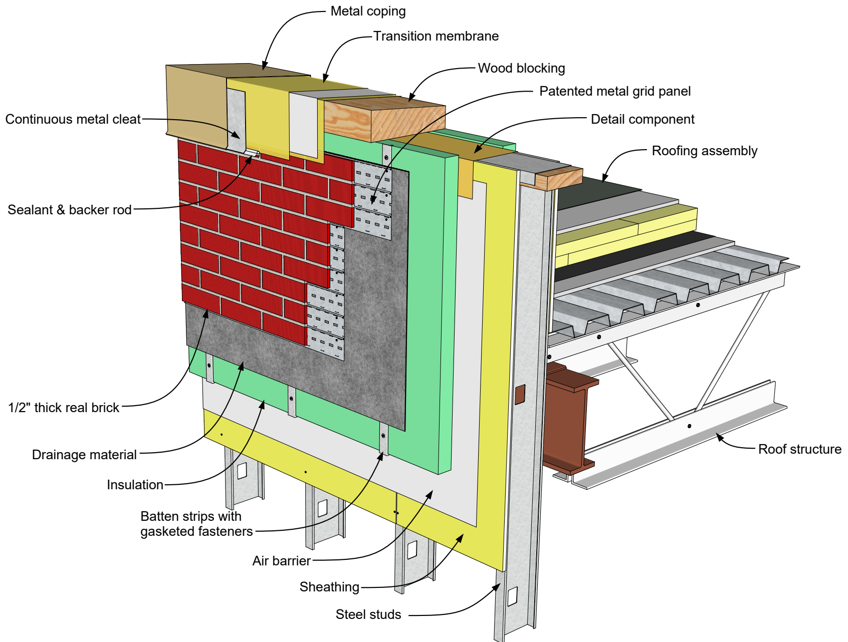
CIS Exterior Wall, Steel Stud Backing | Top of Wall Detail 05.03.06 Rev. 12/26/18
