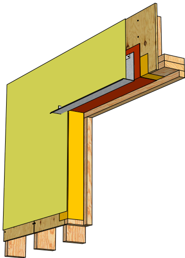
06. Air barrier
