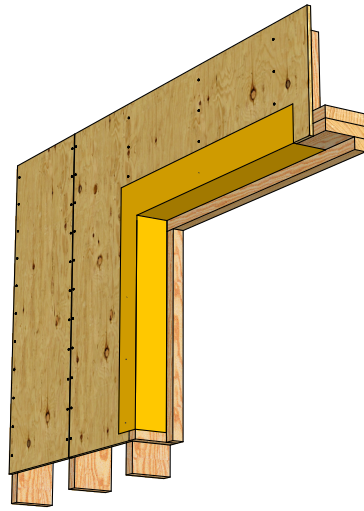
02. Transition membrane
