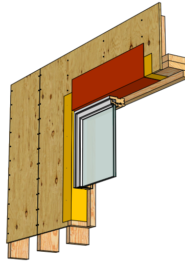
04. Window assembly
