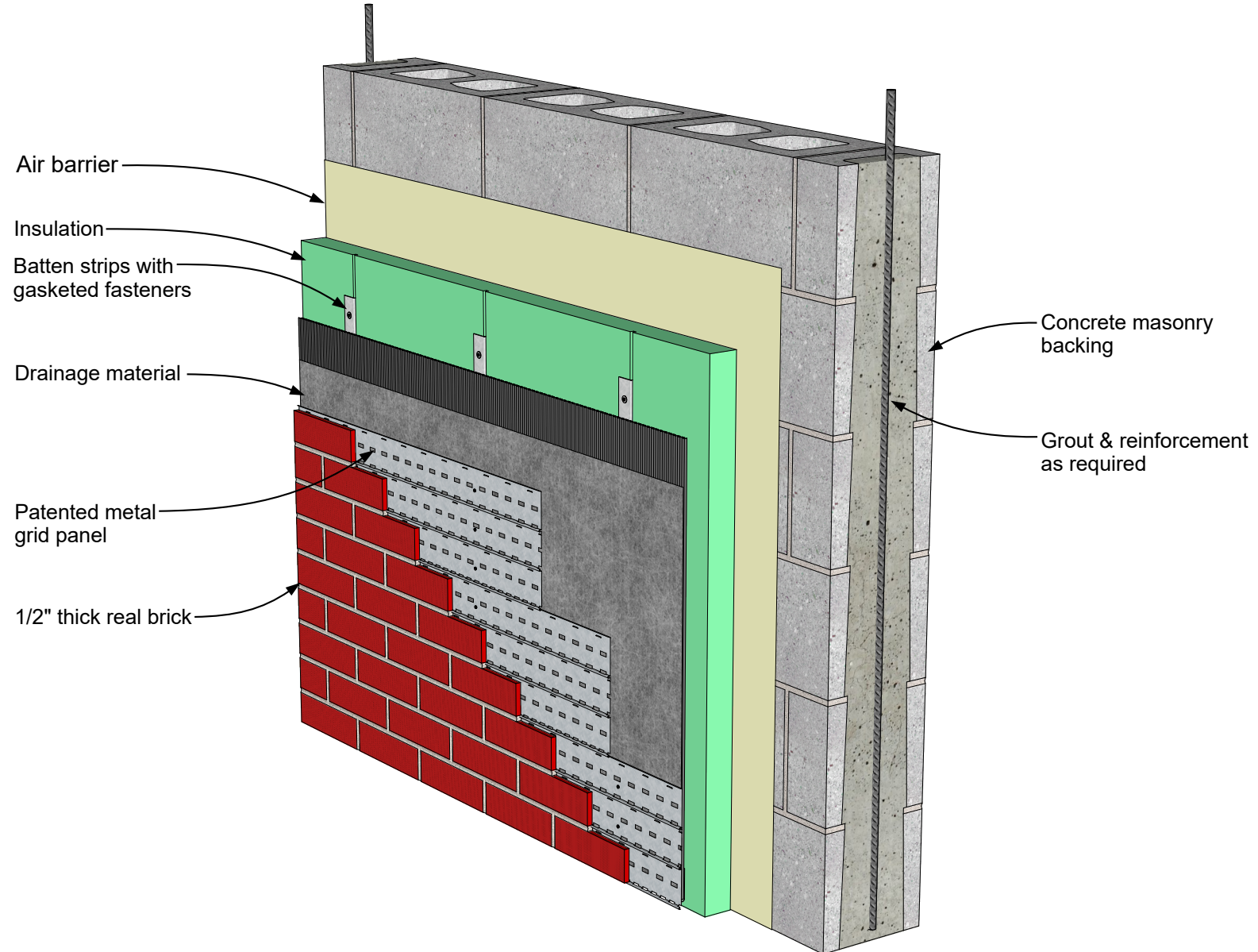
CIS Exterior Wall System, CMU Backing Detail 05.01.00 Rev. 01/12/19
