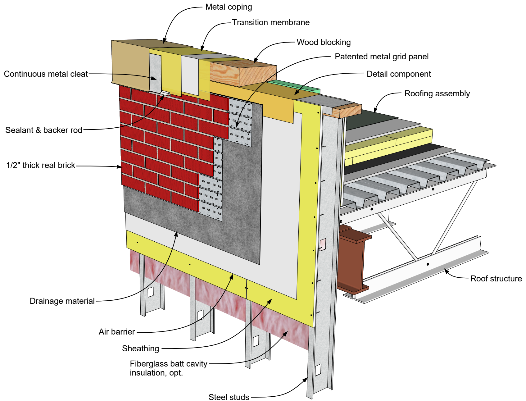
MCS Exterior Wall, Steel Stud Backing | Top of Wall Detail 03.03.06 Rev. 01/27/19
