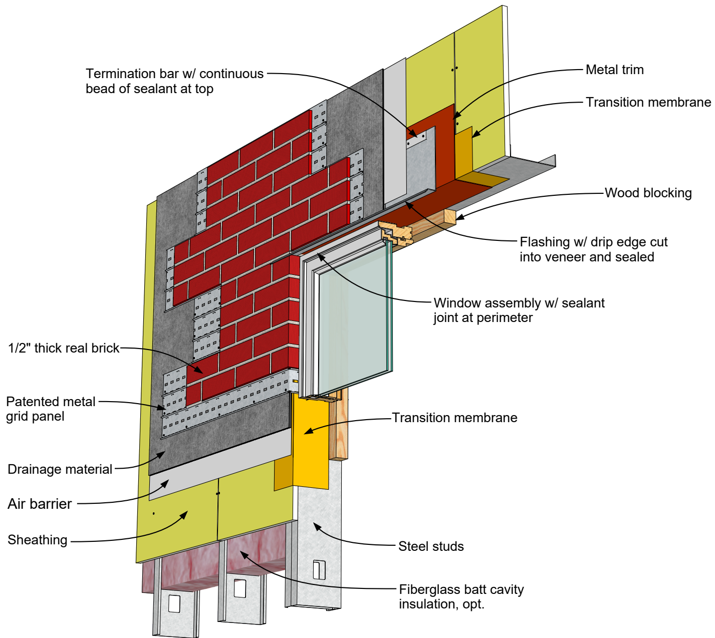
MCS Exterior Wall, Steel Stud Backing | Window Head Detail 03.03.03 Rev. 02/10/19
